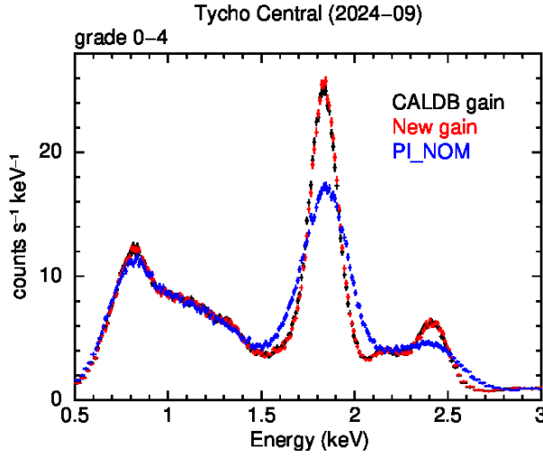
Figure C.5: Comparison of the observed and trap-corrected PC grade 0 – 4 spectra of the Tycho SNR taken in 2024-September, showing the improvements obtained when trap corrections are applied. The FWHM of the Si-K \alpha line is 274 \pm 25 eV for the uncorrected spectrum (blue) and 171 \pm 15 eV for the trap-corrected spectrum using the new gain (red), compared with 174 \pm 15 eV with the previous gain (black).
