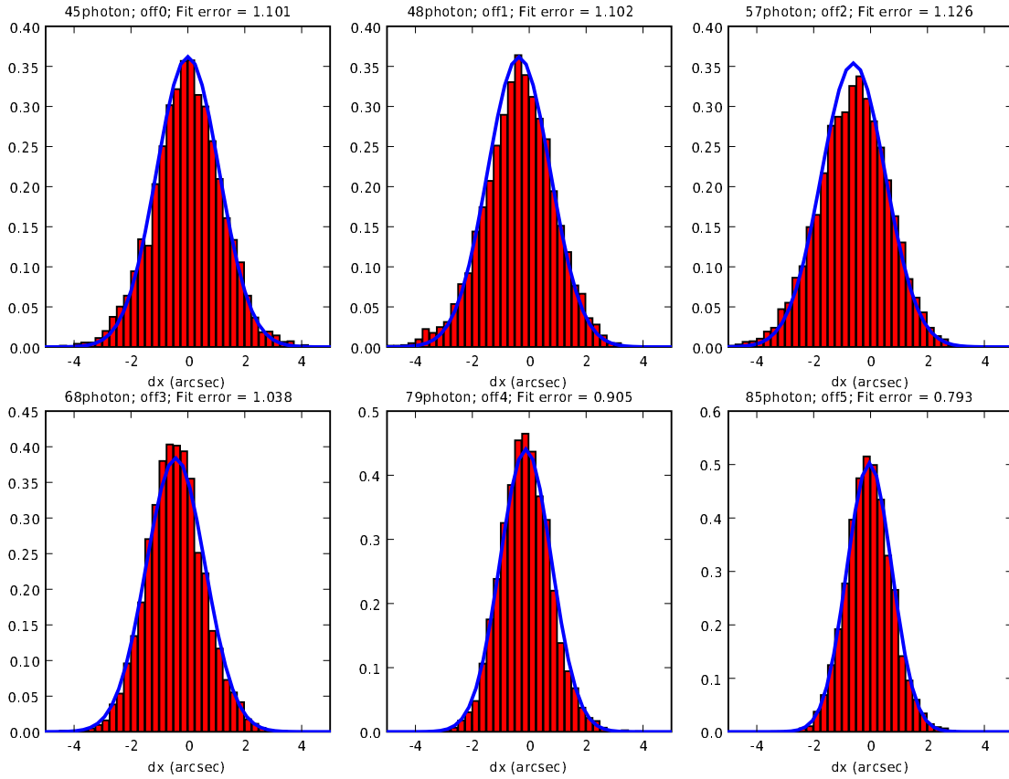
Fig. 4. Distribution of residuals obtained in simulations of XRT images when a non piled-up source is located near 5 bad columns. From top-left to bottom-right, the bad columns are systematically offset by 0, 1, 2, 3, 4, 5 XRT pixels from the centre of the PSF. The red histograms show the distribution of differences of the simulated positions from the input position, while the blue curve is the Gaussian average fit error. The poorest case (a 2 pixel offset) yields a 0.6 arcsecond mismatch which is added as an additional systematic error when this offset occurs. There were 5000 simulations per run, for a source of 100 counts intensity.
