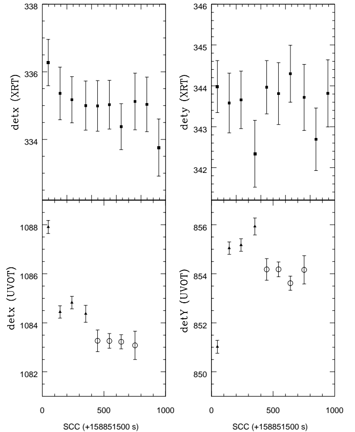
Fig. 2. A comparison of the detector coordinate positions of the XRT (upper panels) and the UVOT (lower panels) as a function of Space Craft Clock (SSC) time for one orbit of observations of 3C279. Filled squares XRT, filled triangles (UVOT – UVW2), open circles (UVOT – UVM2). One XRT pixel is 2.36 arcseconds to a side. One UVOT pixel is 0.5 arcseconds to a side.
