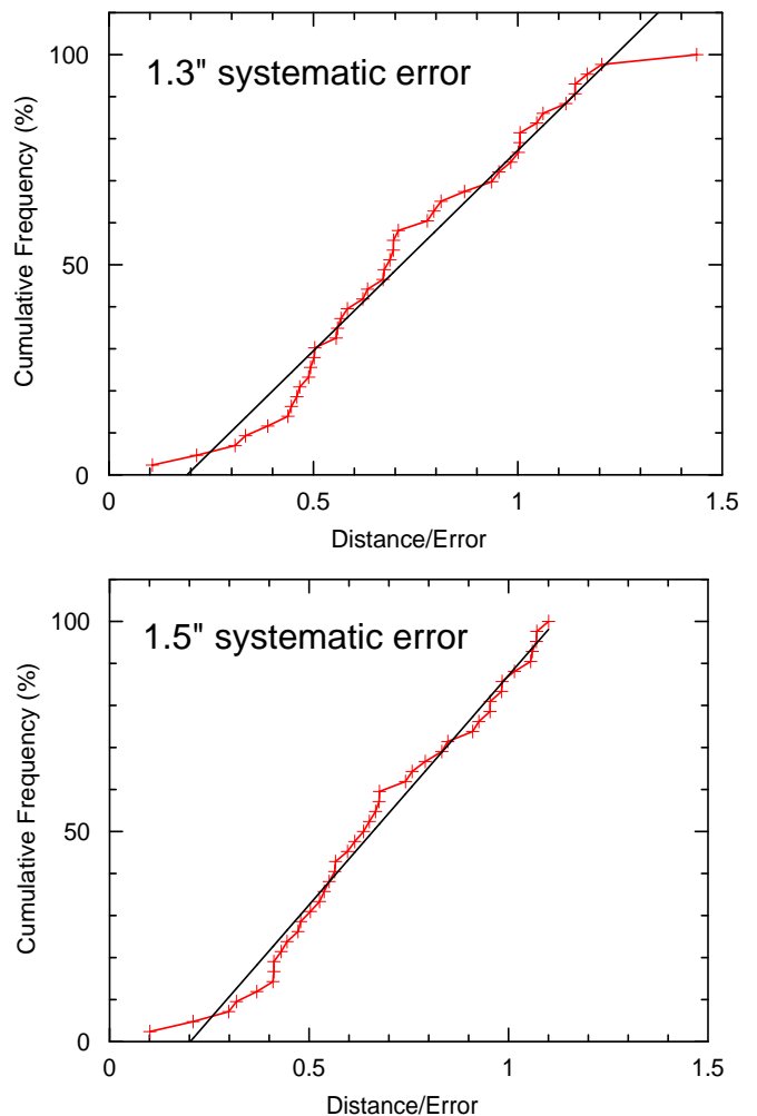
Fig. 9. Results of comparing the UVOT-enhanced XRT GRB positions with the UVOT GRB positions. The upper panel shows that when the 1.3'' systematic error derived from the UVOT-XRT mapping is included in the 90% error radius, the positions agree \sim 80\% of the time. After increasing the 1.3'' systematic to 1.5'' (lower panel), the positions agree 90% of the time.
