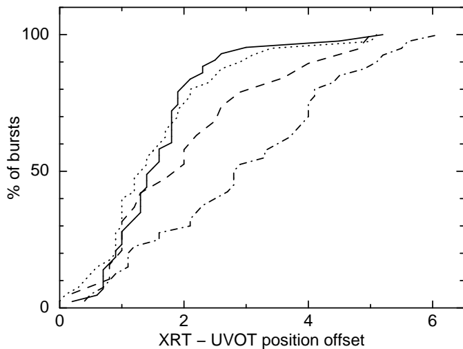
Fig. 8. The cumulative distribution of XRT position offsets (in arcseconds) with respect to 40 UVOT GRB positions available in the literature. Solid-line: UVOT-enhanced XRT position offsets, the result of this work. Dot-dashed line: 'Refined' XRT position offsets, as derived in ground analysis and published in GCN circulars and the Swift data table at http://swift.gsfc.nasa.gov/docs/swift/archive/grb_table/ . Dashed line: astrometrically corrected XRT positions at \approx 24 hours (Butler 2007). Dotted line: final astrometrically corrected positions from deep XRT images (Butler 2007).
