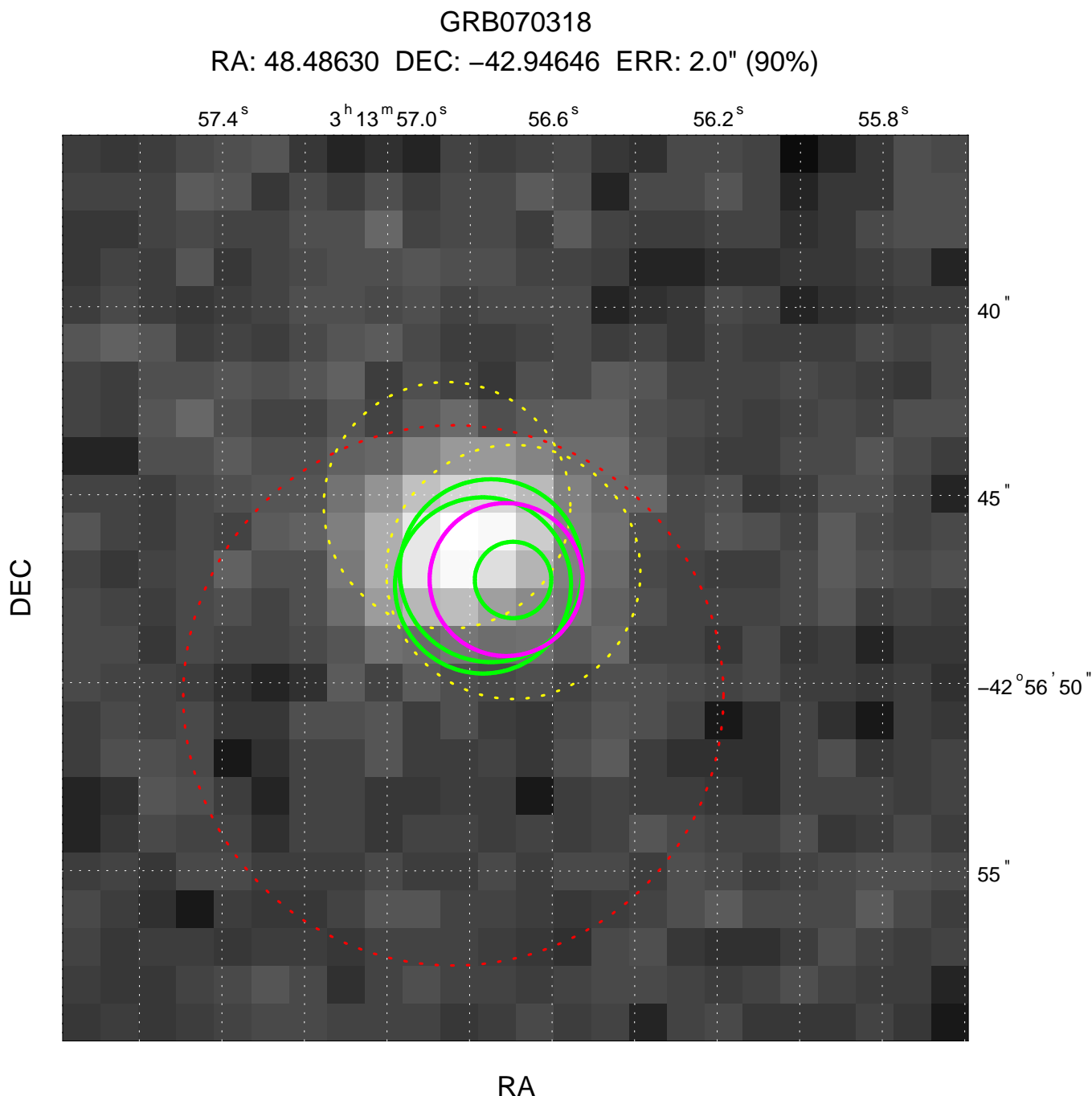
Fig. 7. An example 25x25 arcsecond UVOT sky coordinate V-band image from the detailed results page for GRB 070318 (see http://www.swift.ac.uk/xrt_positions/00271019/image.php for details). The final position (magenta) is based on 3 overlaps (green). One further overlap was rejected as the fit contains fewer than 10 photons (dashed red), and two were rejected as the astrometric correction was considered too large (dashed yellow).
