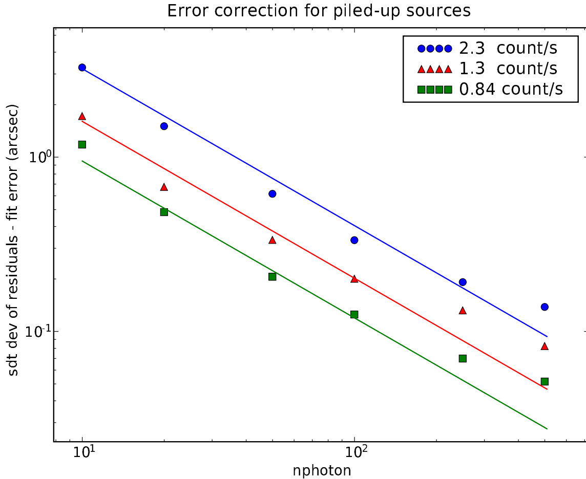
Fig. 6. The error correction term, \epsilon , for simulated piled-up sources fitted with a non piled-up PSF. The solid lines represent the best fit parameterisation of the error correction curve (see text for details).
